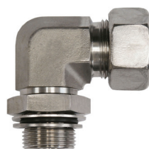
WEE-M MBT-Male Metric Parallel Adjustable 90 Degree
