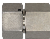
EGVD-BSPP-f Female Metric Swivel-Female BSPP Straight
