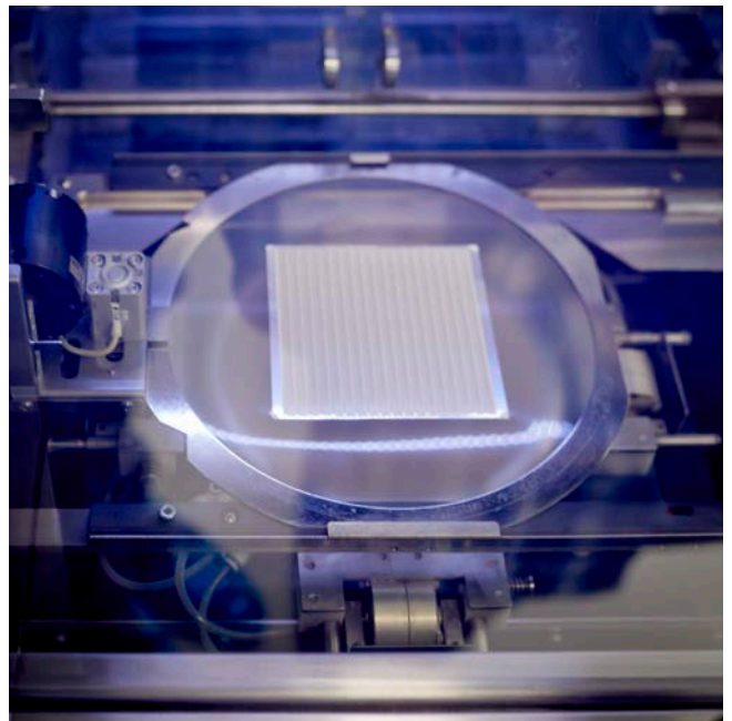
Sensor substrate in dicing machine
